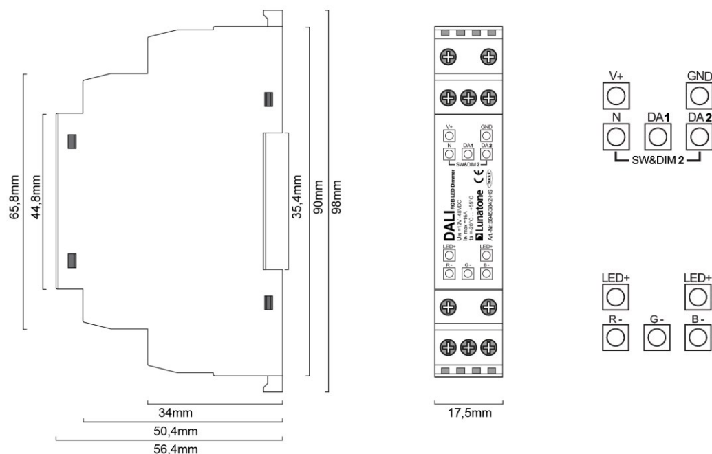
dimensions DIN rail Version 16A Art.Nr.: 89453842-HS
