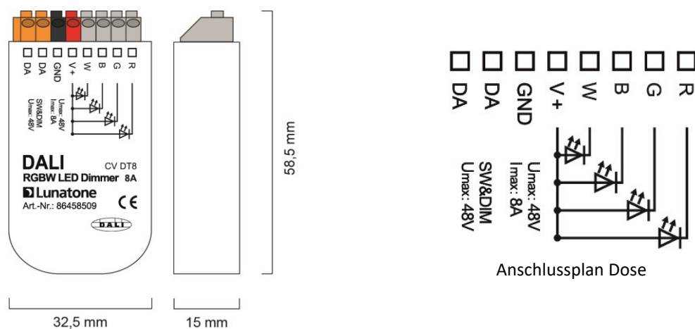
dimensions back box Version 8A Art.Nr.: 86458509
