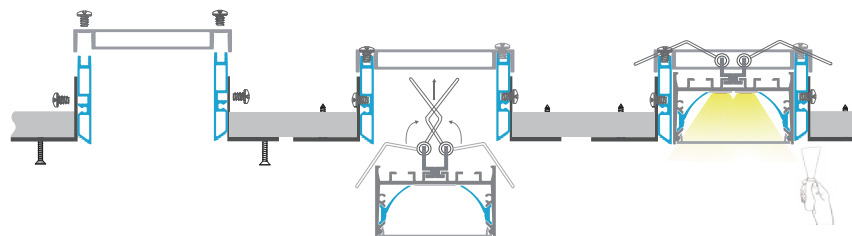
Joiners 120°A Code: J-120A
