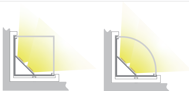
Adjustable Clip (0-222° rotation) Code: AC4-Clip-A
